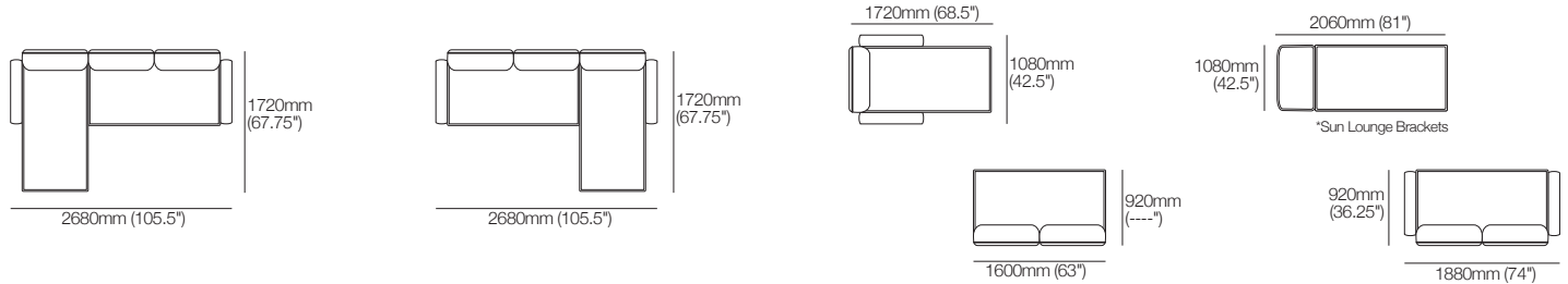
Package: Delta Coast Outdoor 3-Seater with Chaise (Package 1) – WeatherWeave Top View Configurations – Standard Position
