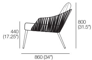
2.5 Seater Side View
